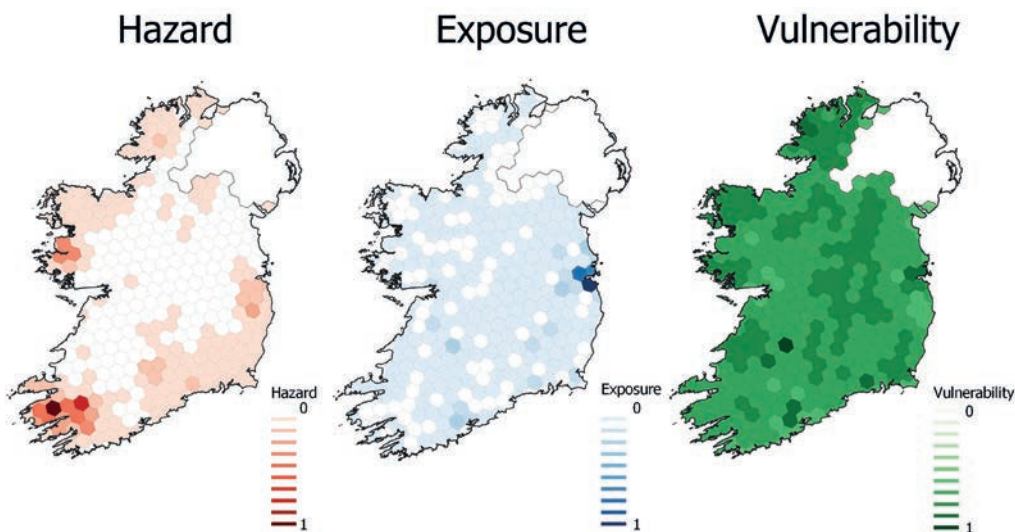
Figure 28. Indexed values of hazard, exposure and vulnerability between 0-1
