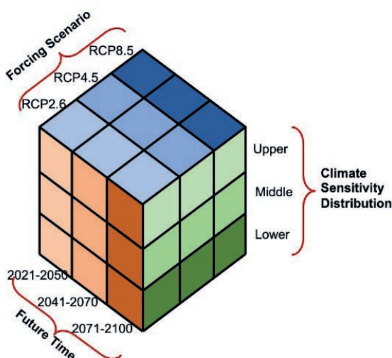
Figure 1. Schematic of how future climate uncertainties can be accommodated in a limited set of possible climates, adapted from Fig.10.9 of CH2018 (CH2018 report, 2018). Each sub-cube shown corresponds to an ensemble of long-term climate simulations. Different RCP emission scenarios represent forcing uncertainty, while the climate sensitivity axis represents response uncertainty.
